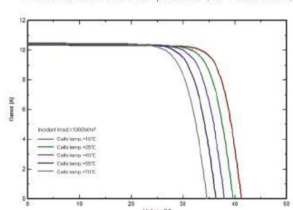
I-V Curve at different temperature ( SPP335N60H )
